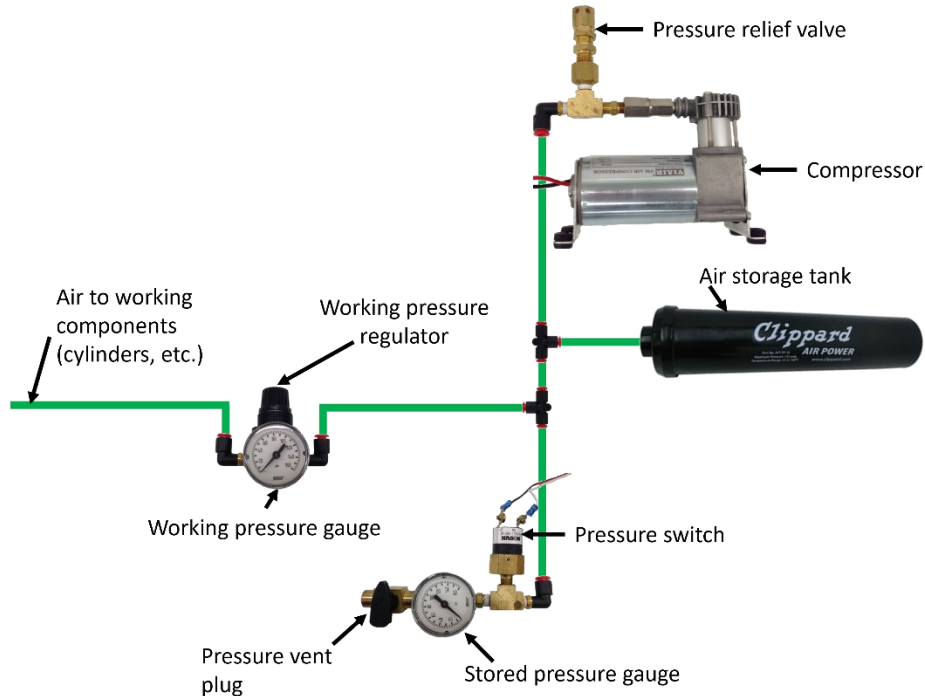
Figure 9-17 Pneumatic circuitry
