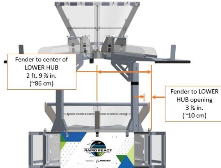
Figure 5-13 Fender geometry
